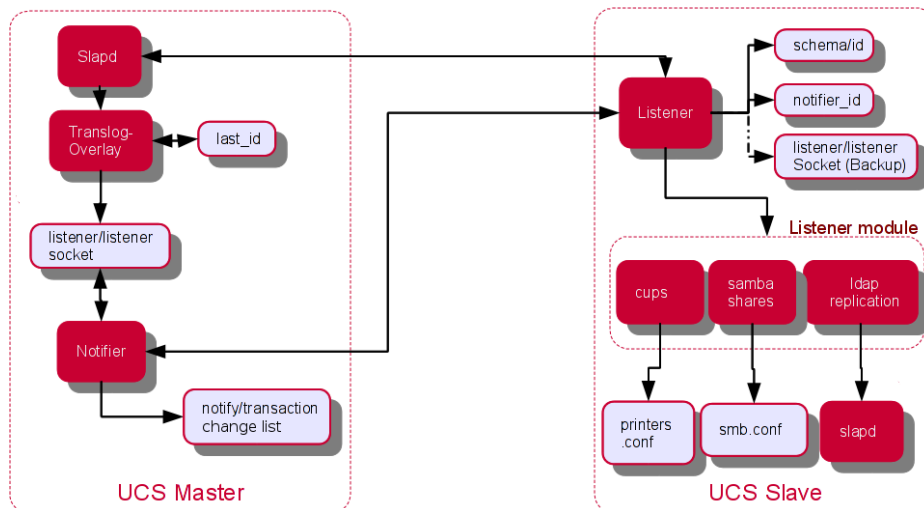
Figure 5.1. Listener/Notifier mechanism
