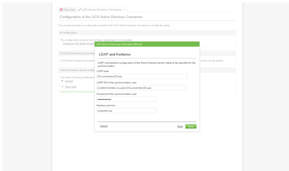
Figure 8.2. Configuring the AD connector in UMC
