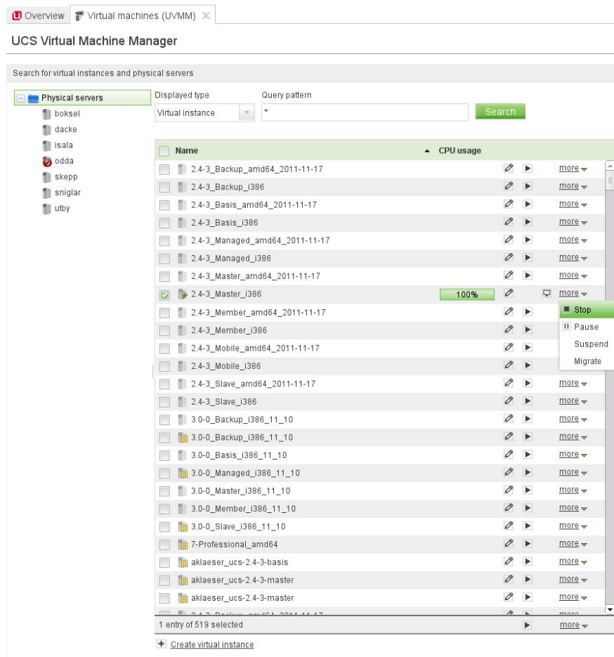
Figure 14.3. Overview of virtual machines
