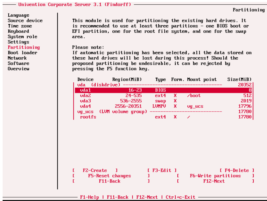
Figure 2.7. Partitioning hard drives
