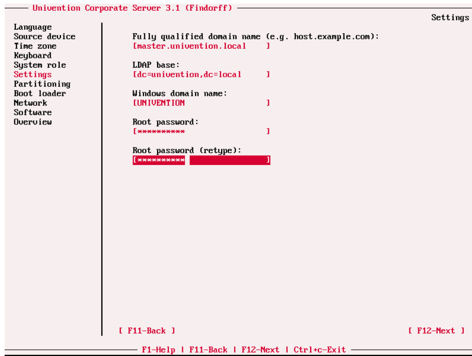
Figure 2.6. Domain settings
