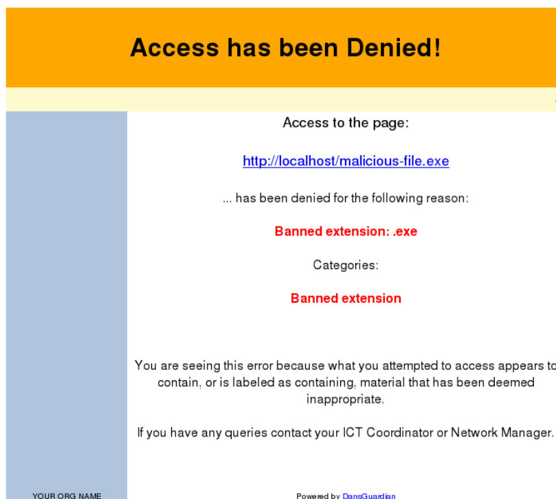
Figure 9.4. Dansguardian blocking a web site
