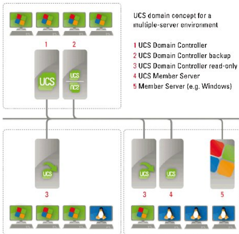
Figure 1.1. UCS domain concept
