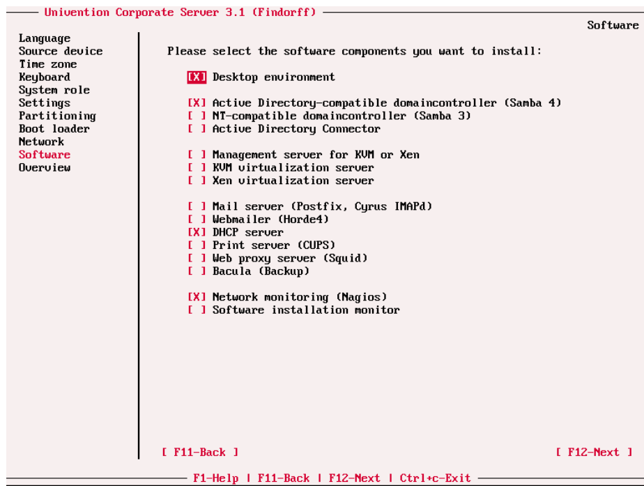
Figure 2.9. Software selection
