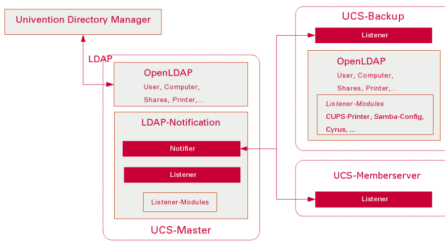
Figure 3.3. Listener/Notifier mechanism
