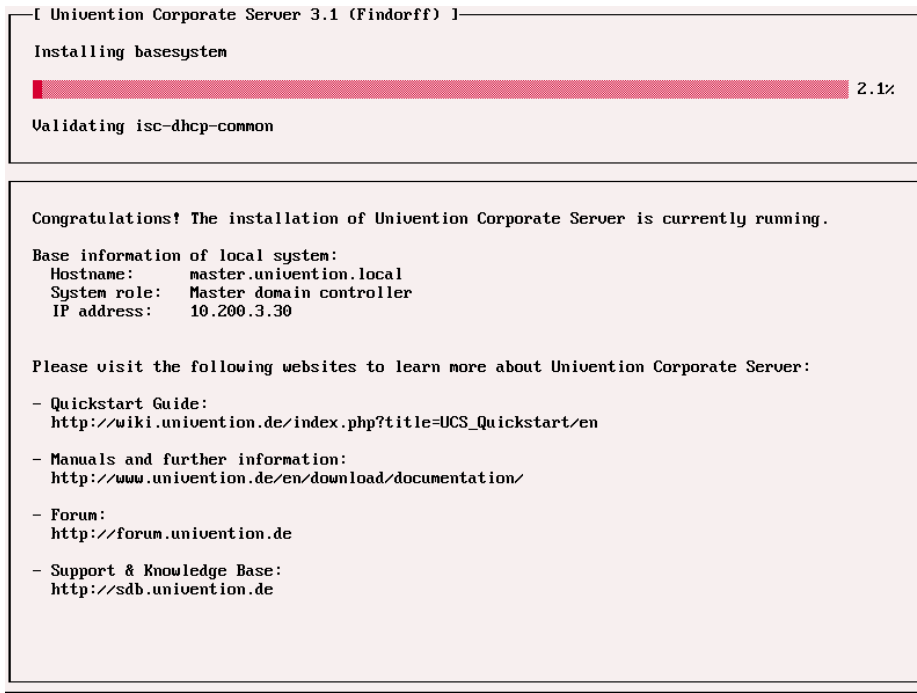
Figure 2.11. Installation progress
