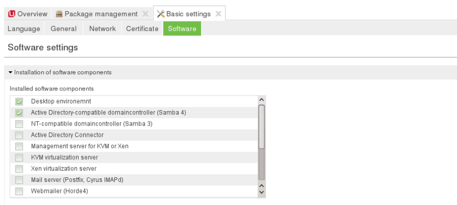
Figure 7.10. Software selection
