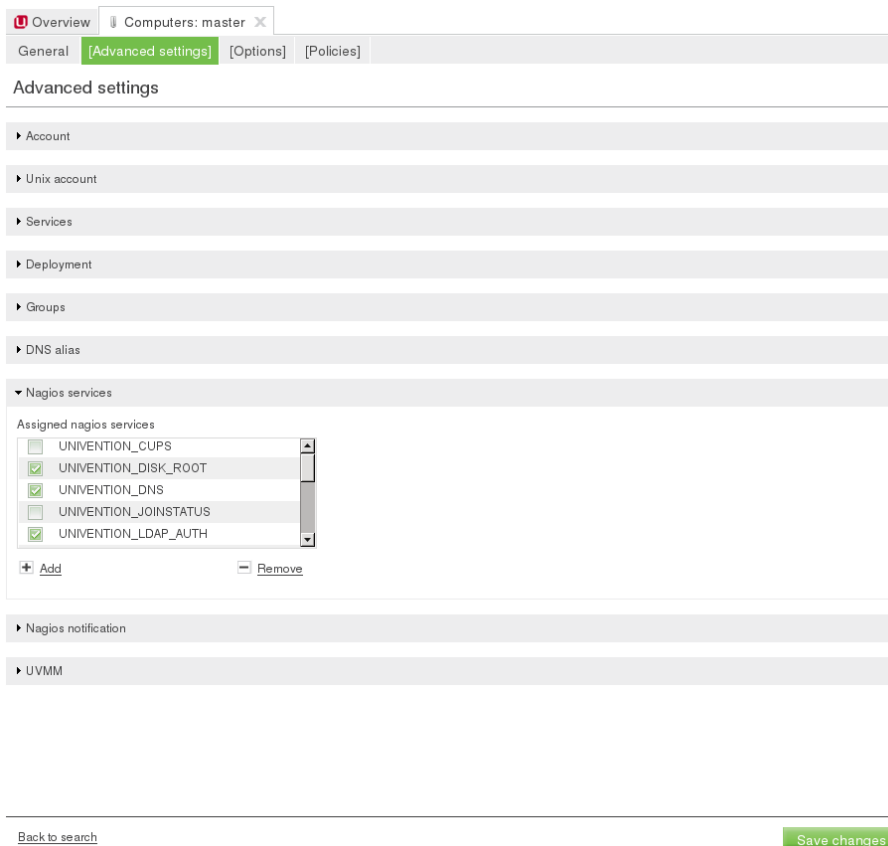
Figure 13.3. Assigning Nagios checks to a host
