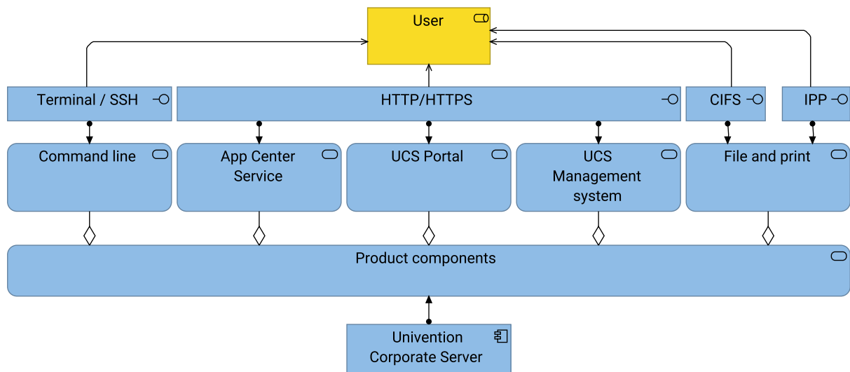
Fig. 4.1: User facing product components of UCS
