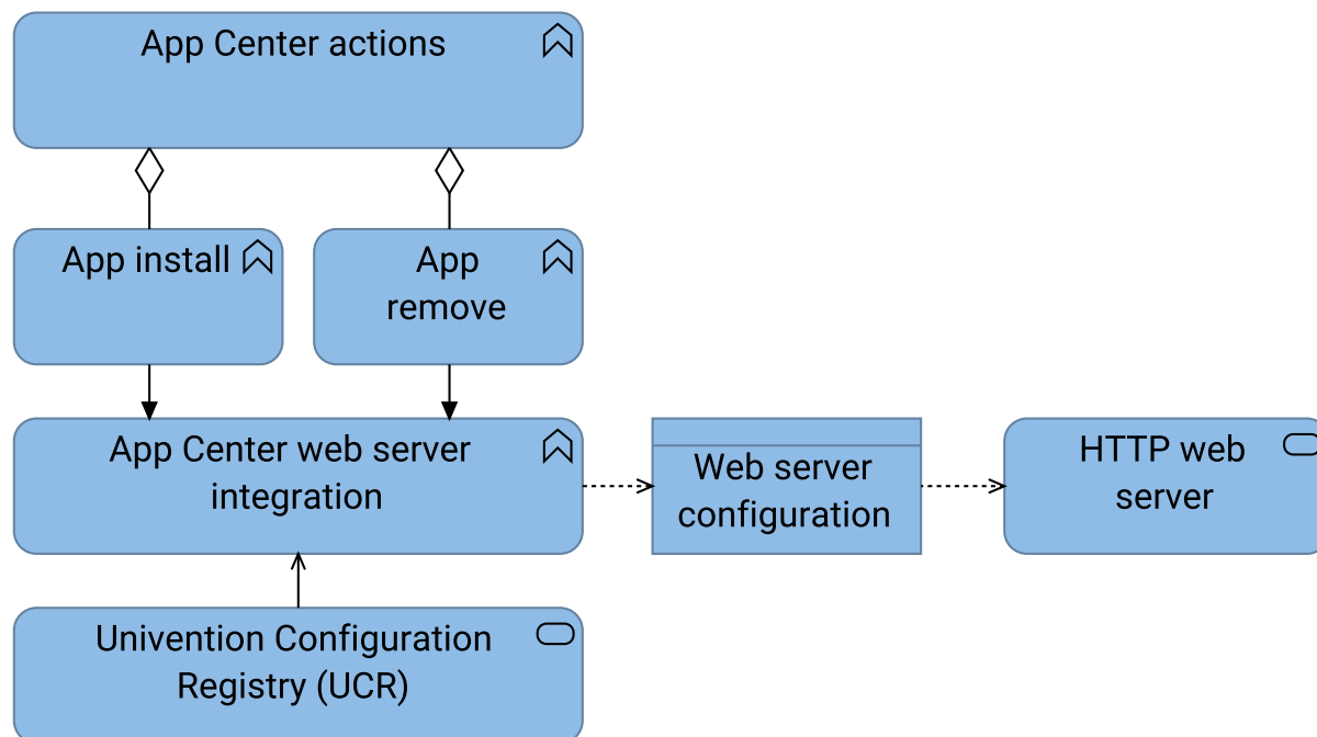
Fig. 5.25: App Center web server integration
