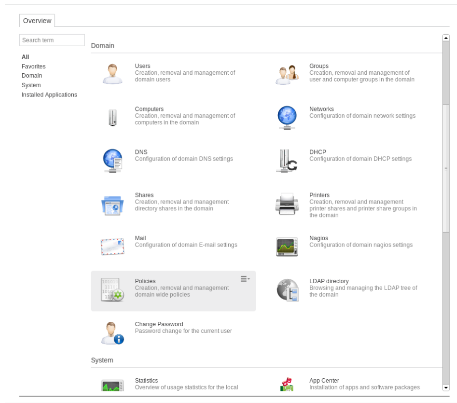
Figure 4.3. Module overview
