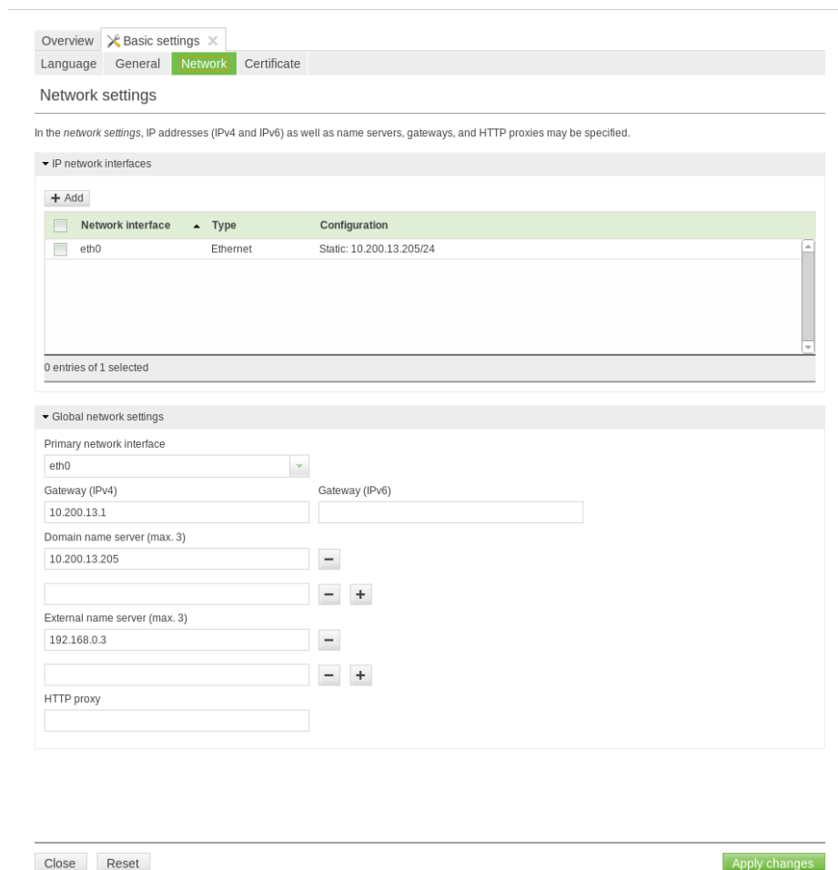
Figure 8.2. Configuring the network settings
