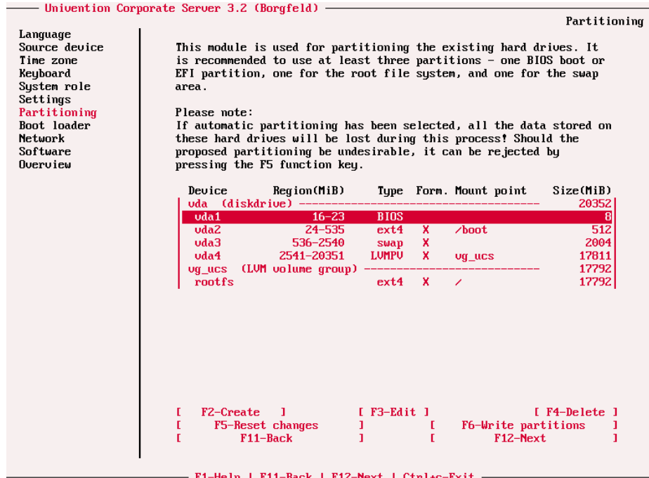
Figure 2.7. Partitioning hard drives
