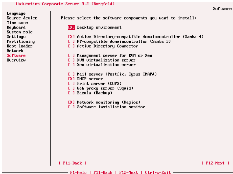
Figure 2.9. Software selection
