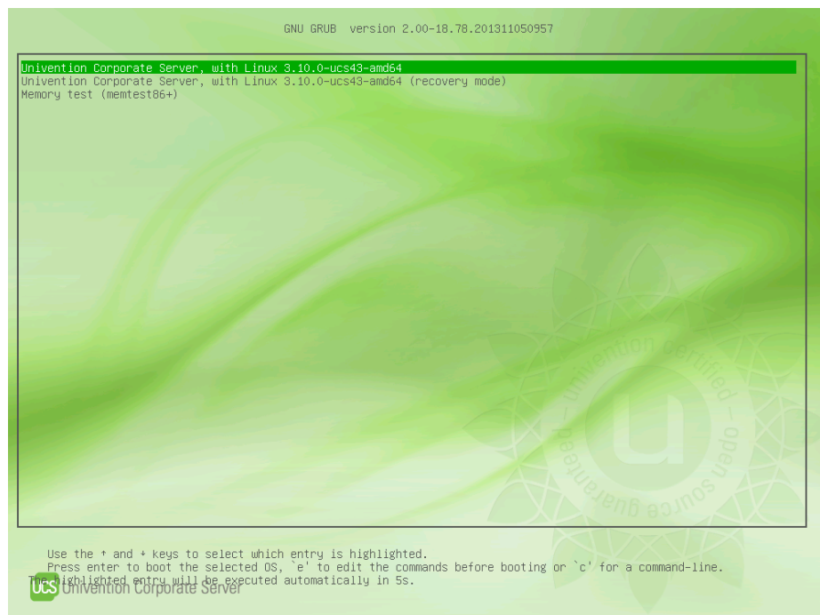
Figure 8.1. GRUB menu
