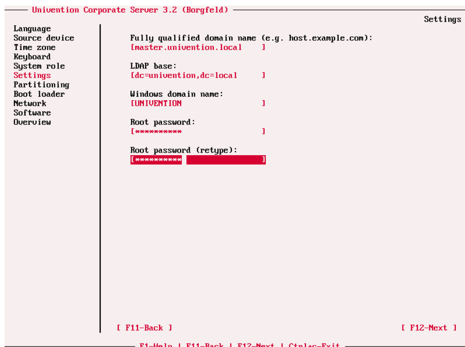
Figure 2.6. Domain settings
