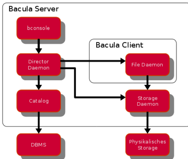
Figure 16.1. Bacula Schema
