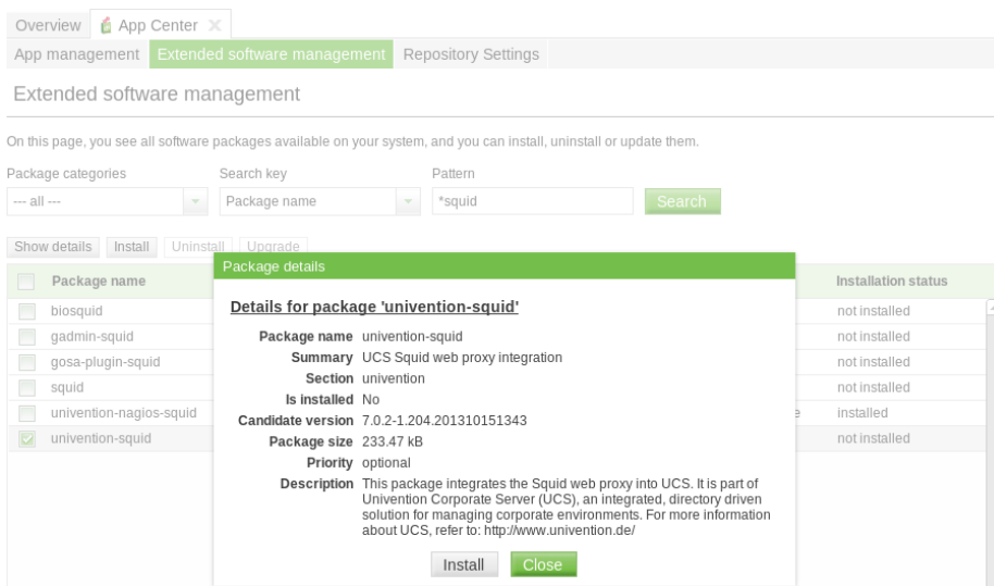
Figure 5.6. Installing the package univention-squid in the Univention Management Console
