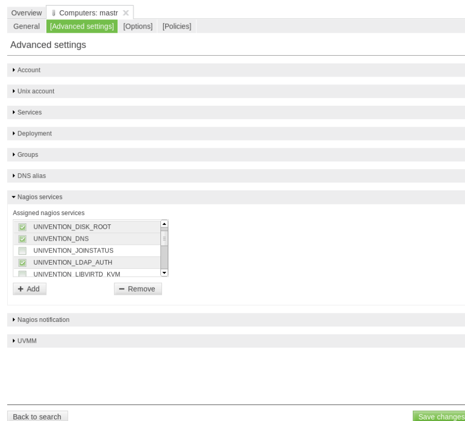
Figure 14.3. Assigning Nagios checks to a host
