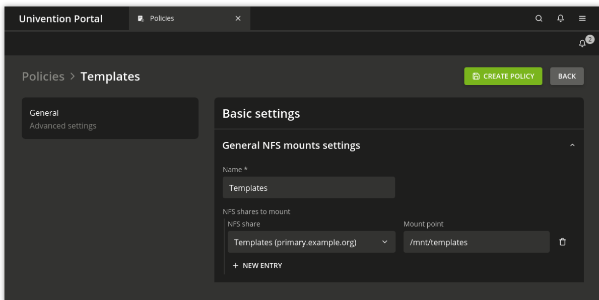
Fig. 8.5: Mounting a NFS share
