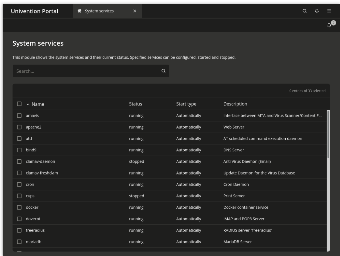
Fig. 8.8: Overview of system services
