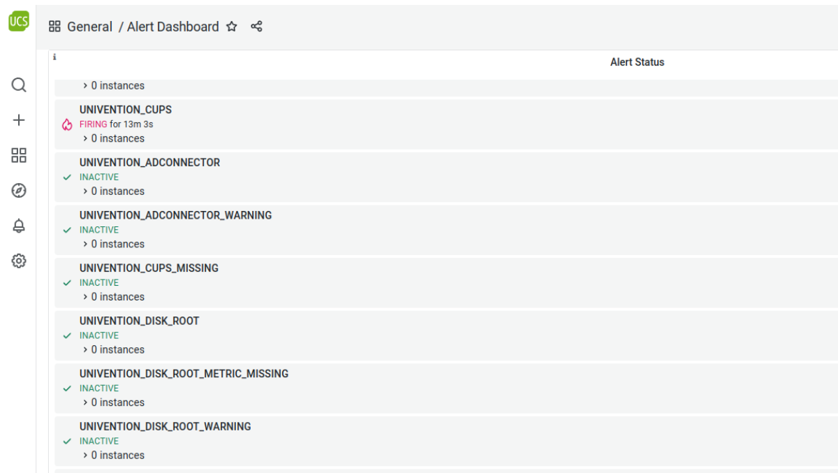
Fig. 15.3: Alert Dashboard
