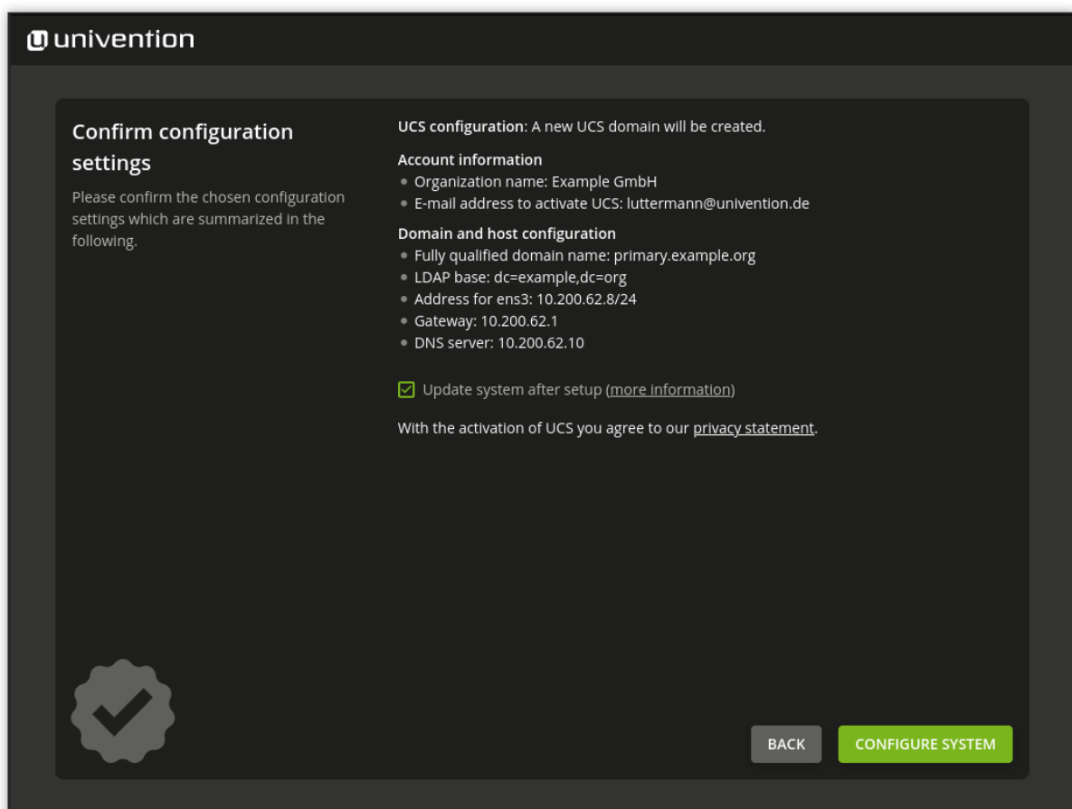
Fig. 2.16: Installation overview
