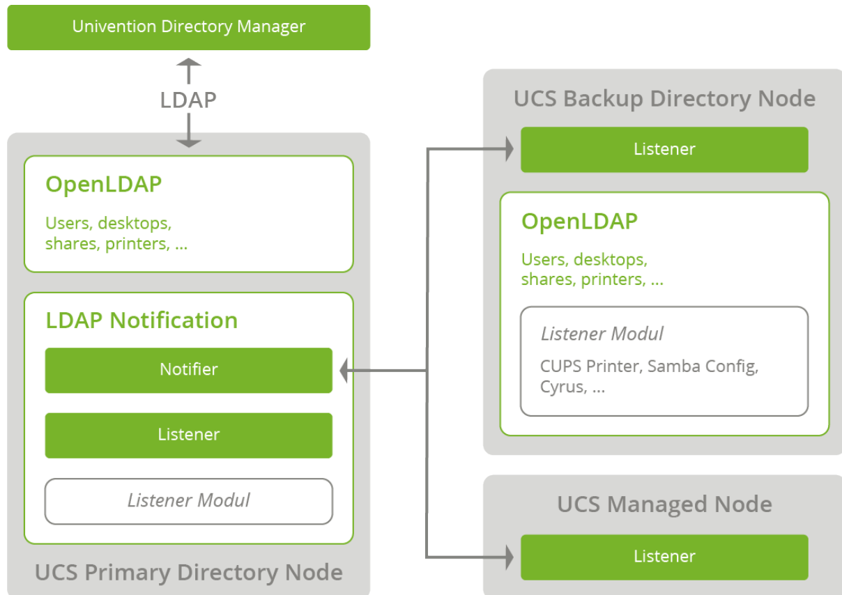
Fig. 3.2: Listener/Notifier mechanism
