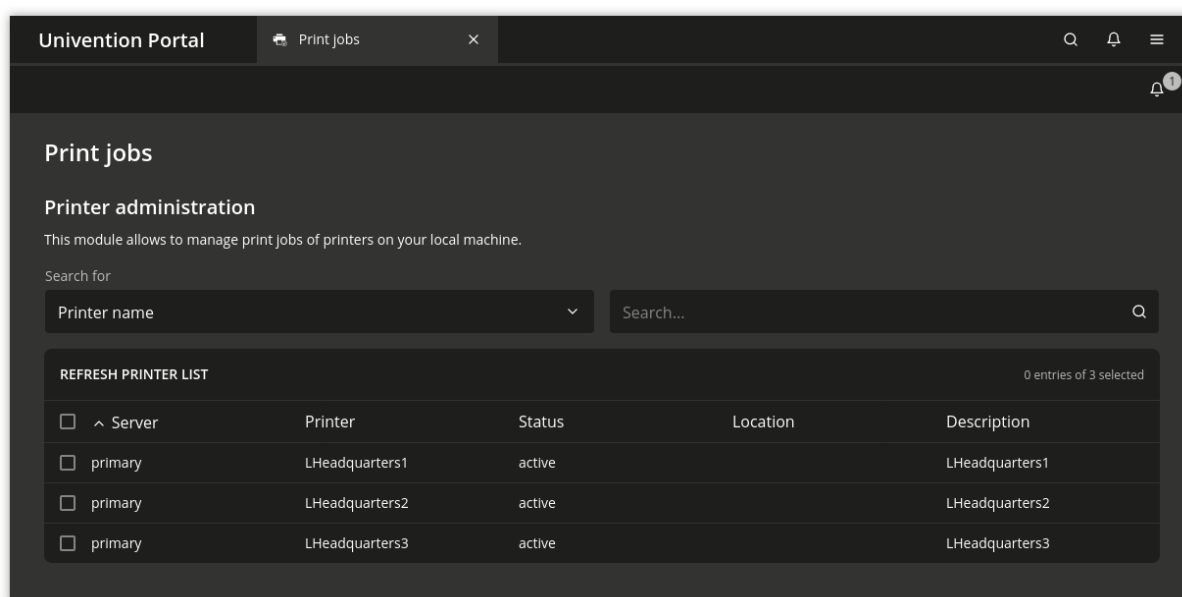
Fig. 13.2: Printer administration
