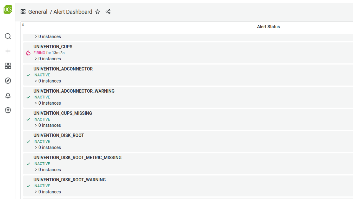
Fig. 15.4: Alert dashboard
