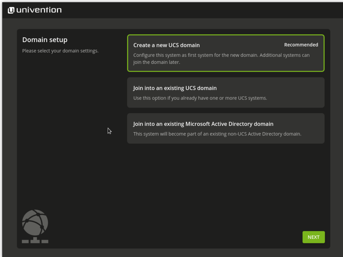
Fig. 2.12: Domain settings
