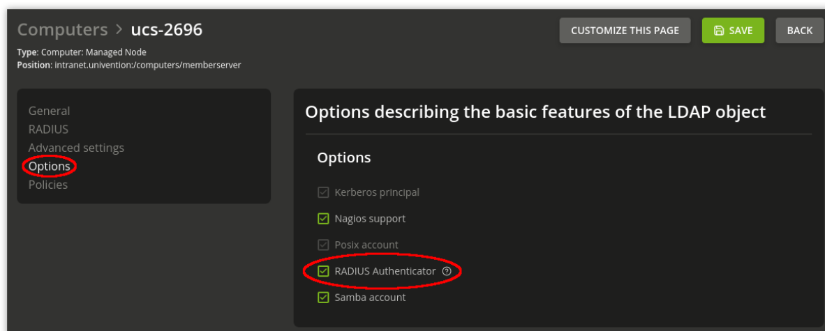
Fig. 11.6: RADIUS option
