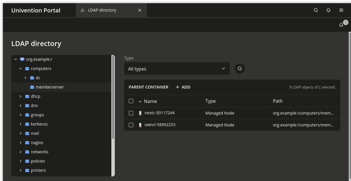
Fig. 4.8: Navigating the LDAP directory
