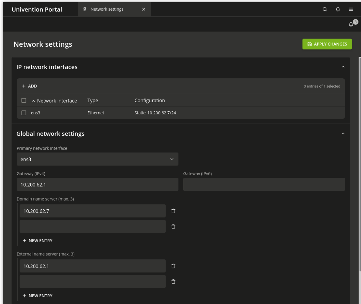
Fig. 8.4: Configuring the network settings
