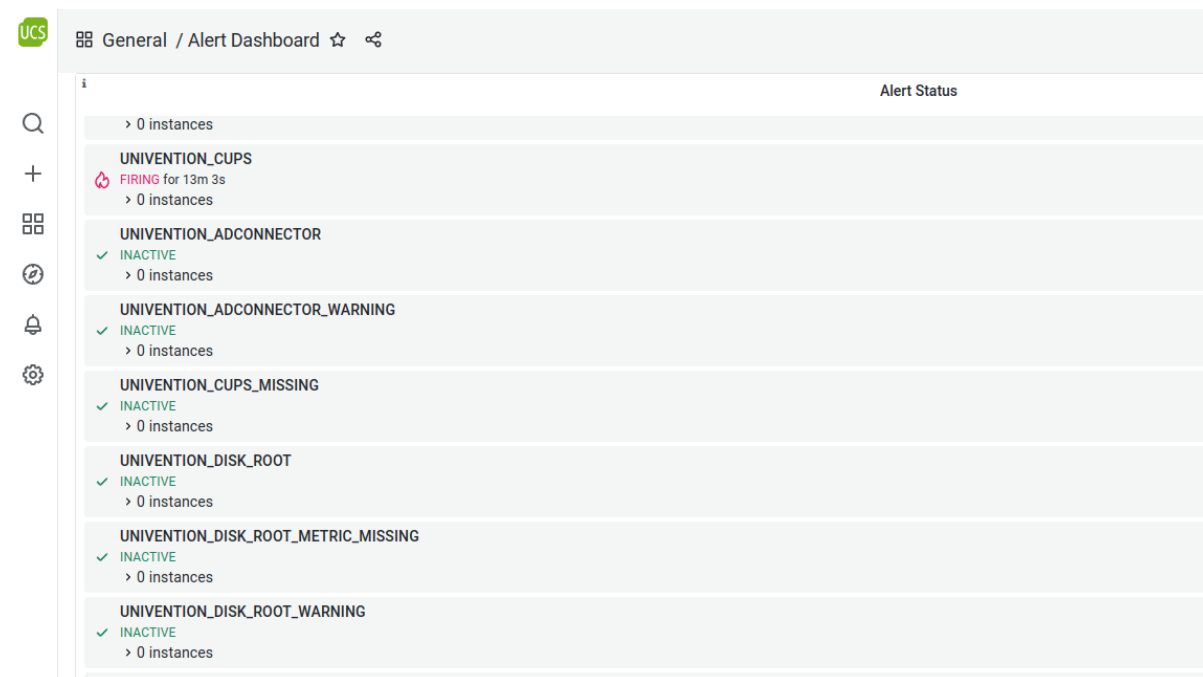
Abb. 15.4: Alert Dashboard
