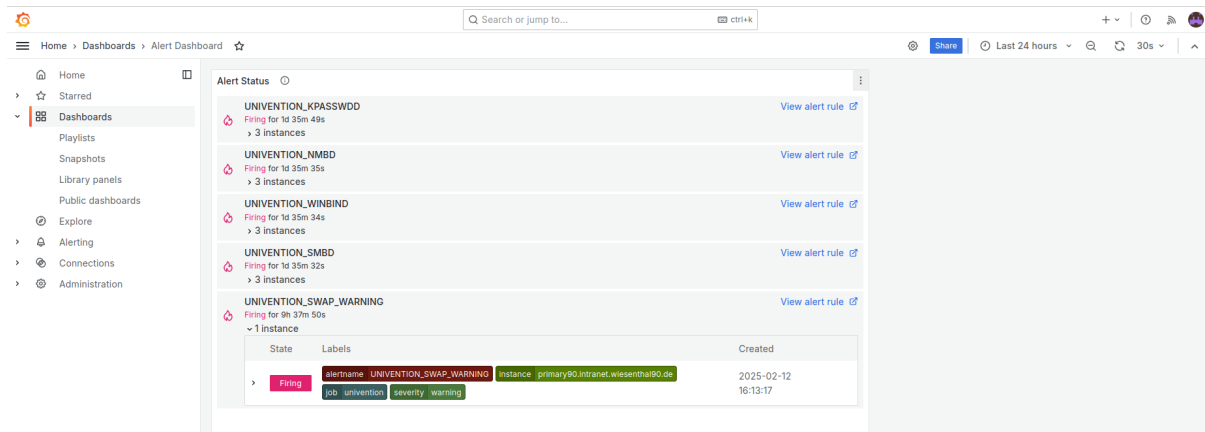
Fig. 15.3: Alert Dashboard
