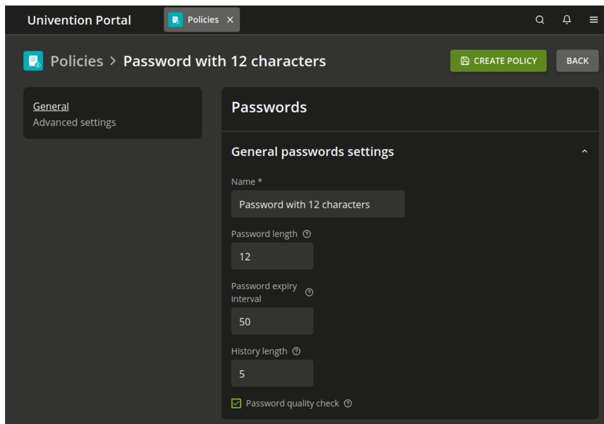
Fig. 6.7: Configuring a password policy
