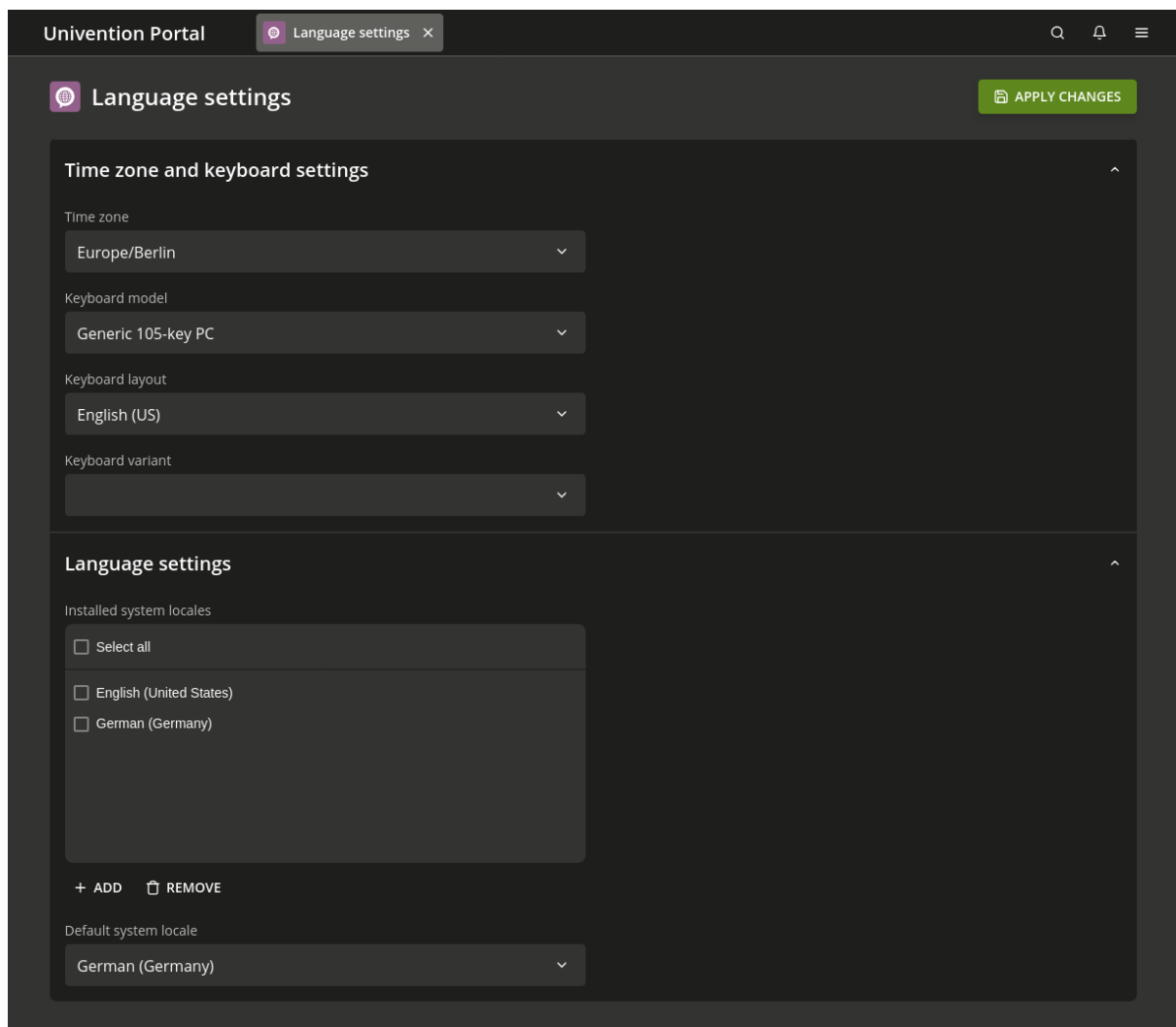
Fig. 8.8: Configuring the language settings
