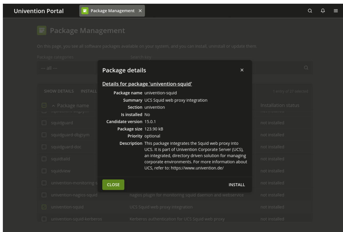
Fig. 5.7: Installing the package univention-squid via Univention Management Console module ‘Package management’
