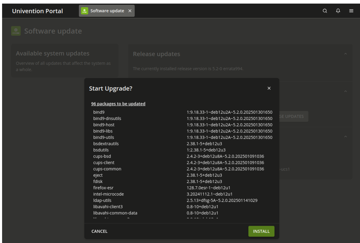
Fig. 5.4: Updating a UCS system via UMC module Software update
