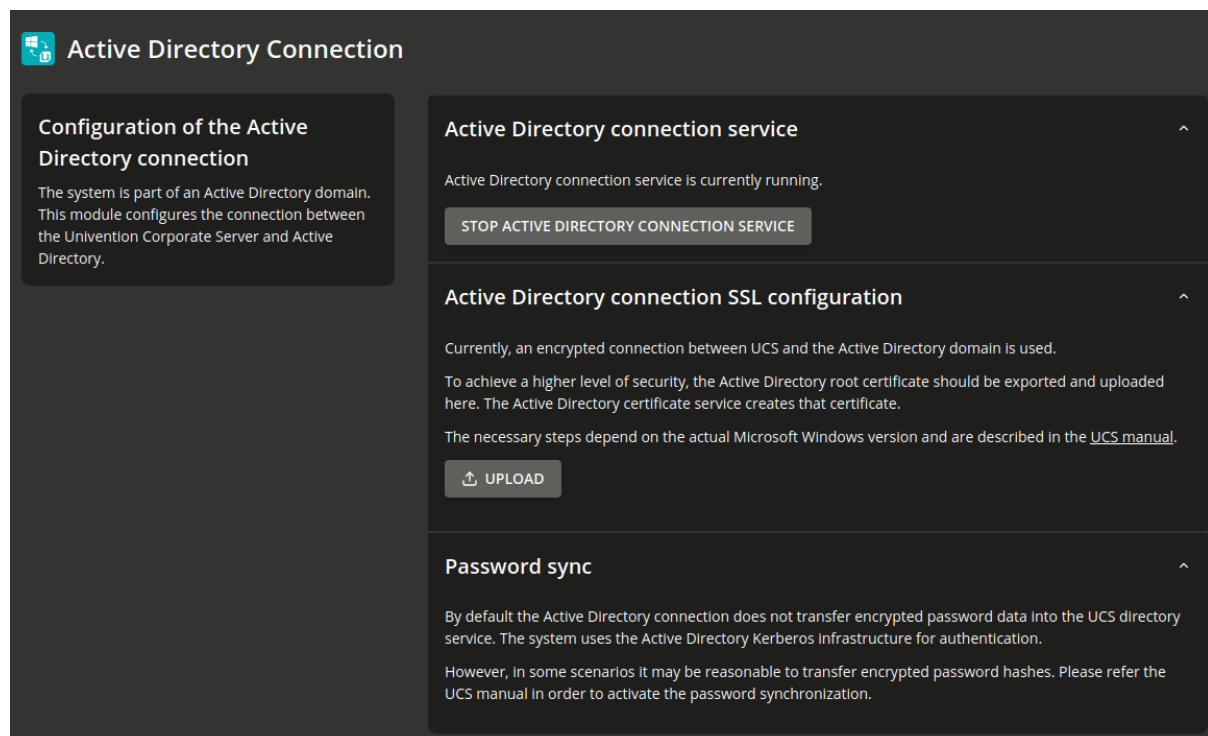
Fig. 9.8: Administration dialogue for the Active Directory Connection
