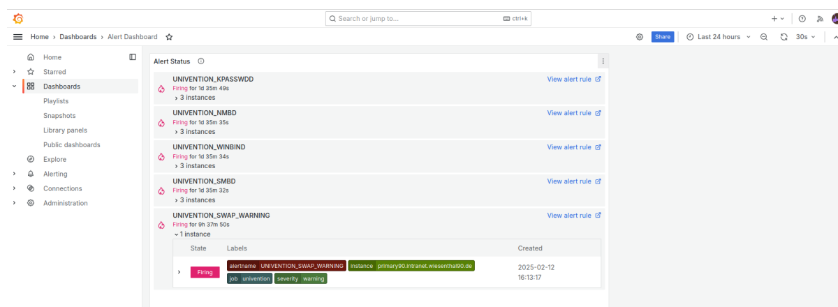
Fig. 15.4: Alert dashboard
