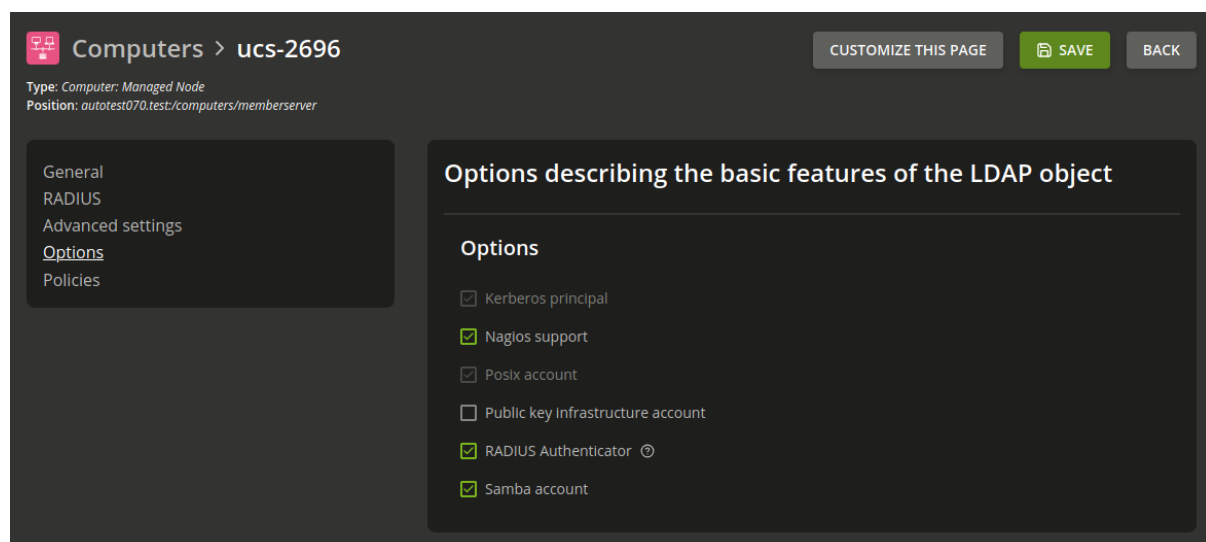
Fig. 11.6: RADIUS option
