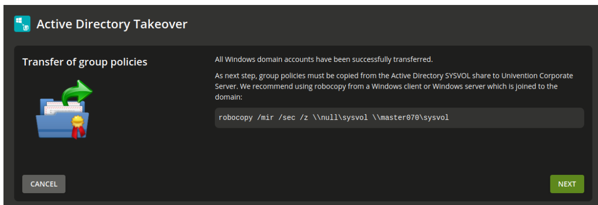
Fig. 9.11: Copying the SYSVOL share
