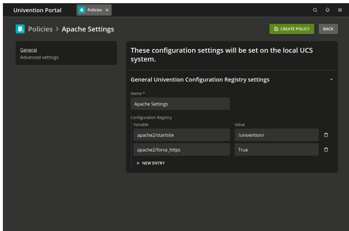
Fig. 8.7: Policy-based configuration of the Apache start page and forced HTTPS
