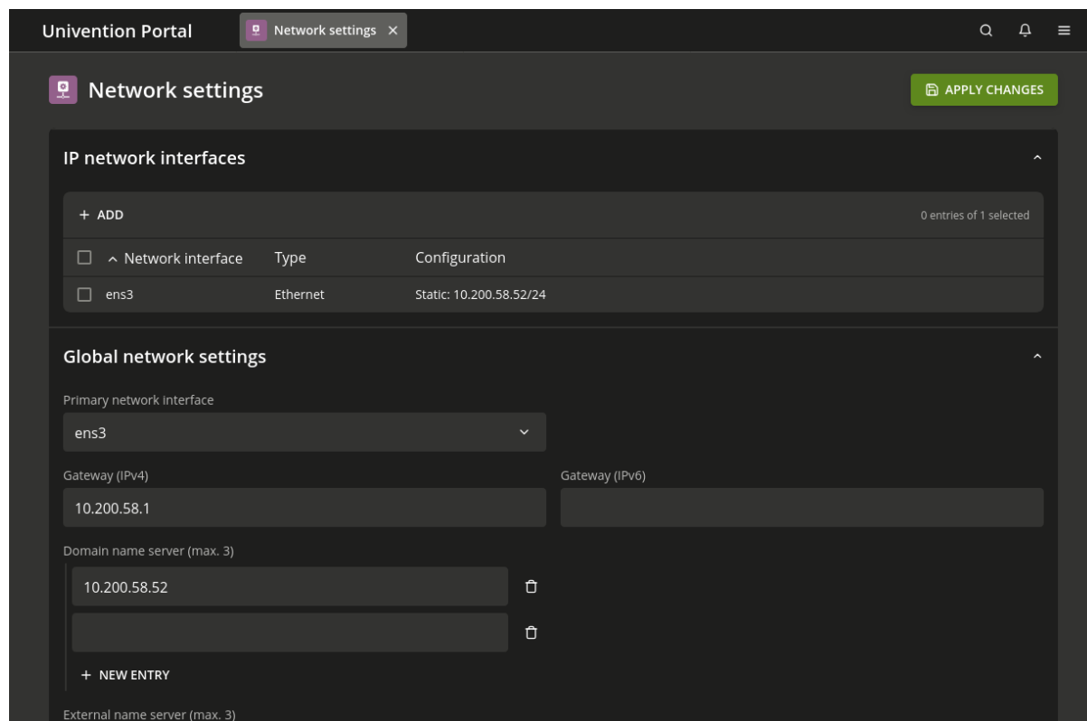
Fig. 8.4: Configuring the network settings
