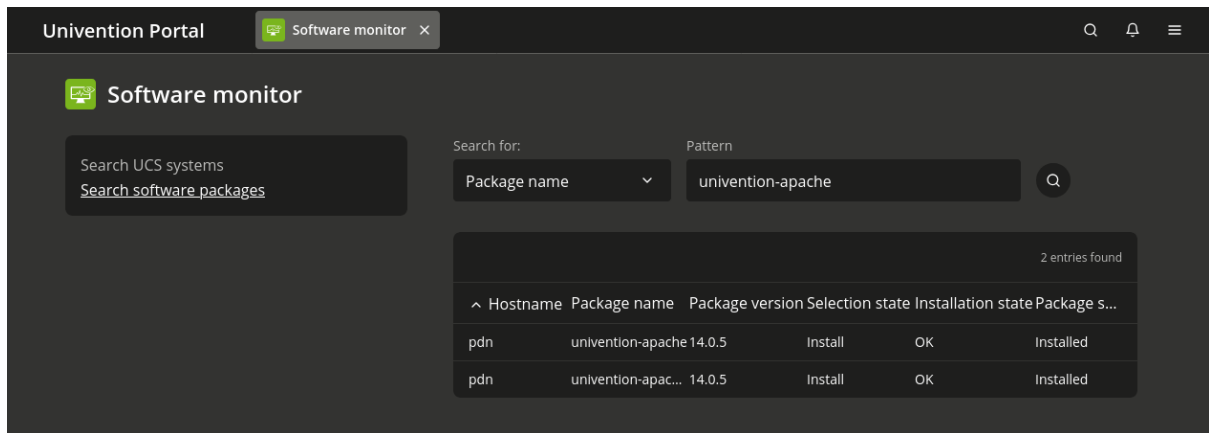
Fig. 5.8: Searching for packages in the software monitor
