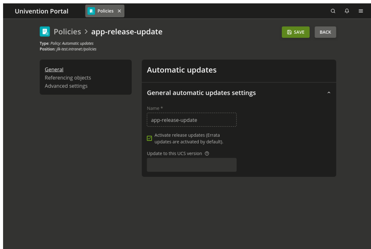
Fig. 5.5: Updating UCS systems using an update policy
