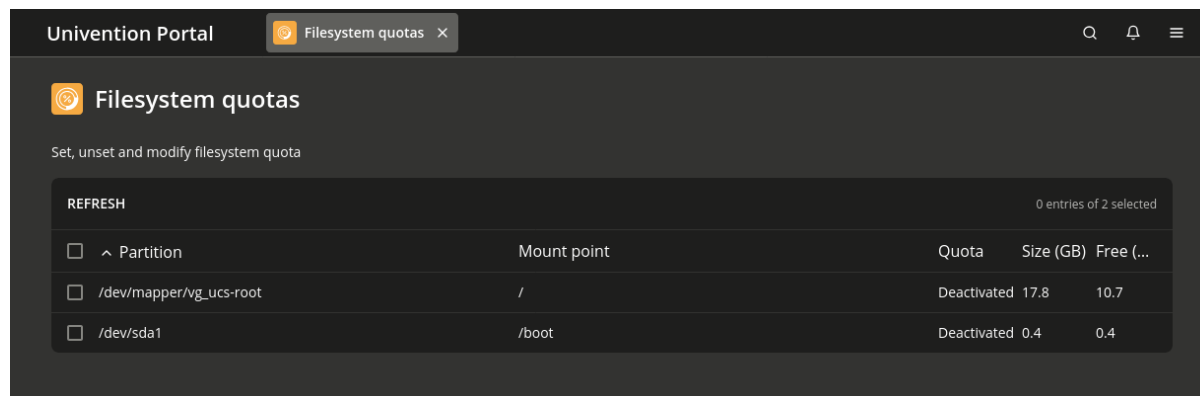
Fig. 12.2: The UMC module File system quotas
