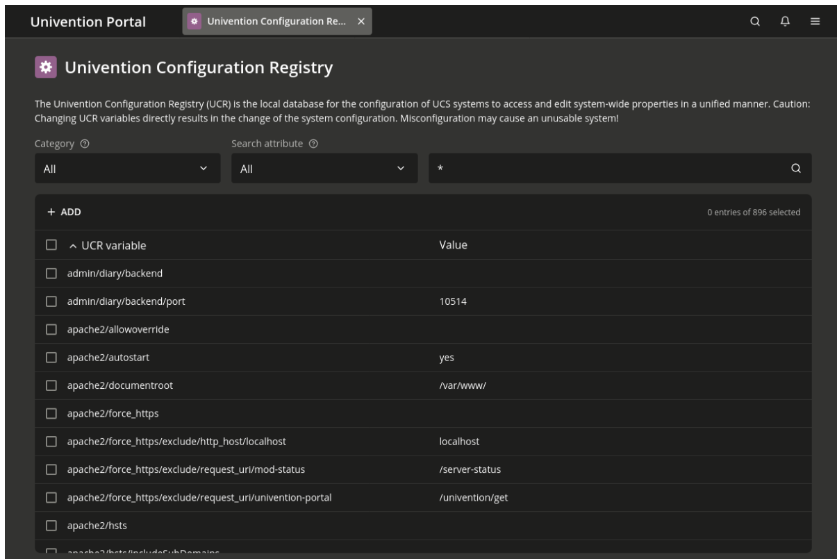
Fig. 8.6: Managing Univention Configuration Registry variables via the UMC
