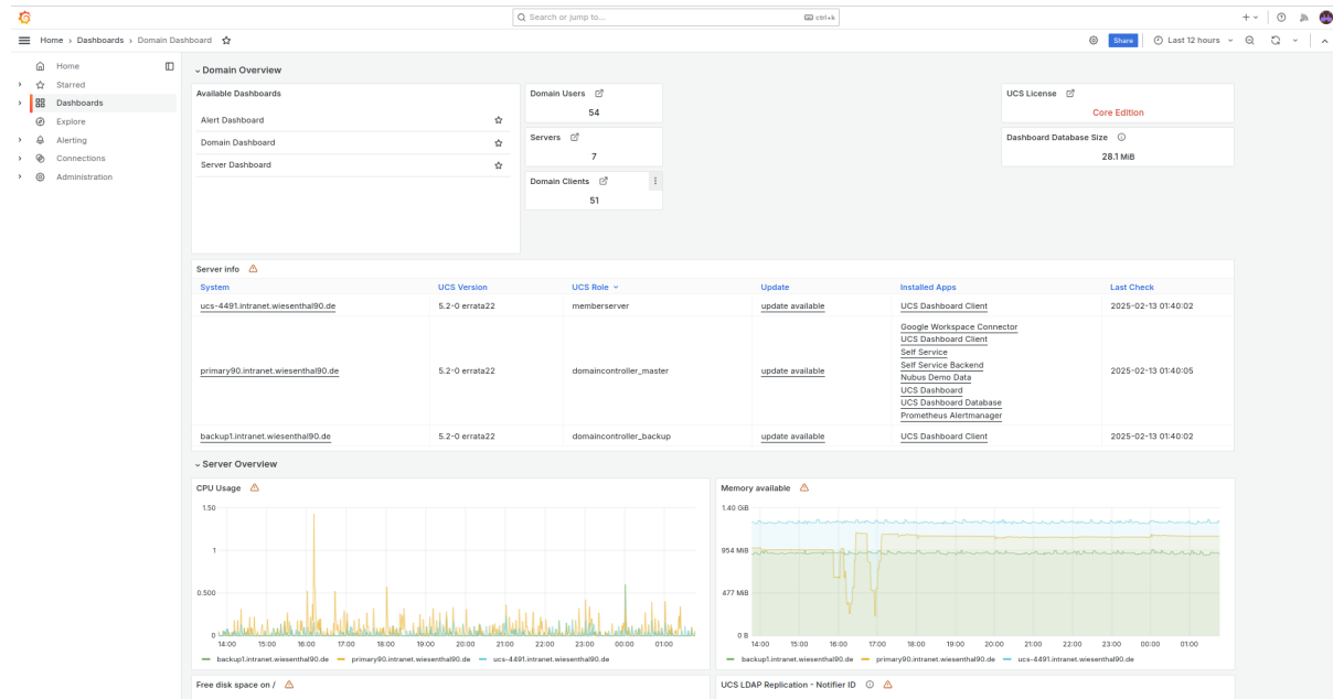
Fig. 15.1: Domain dashboard
