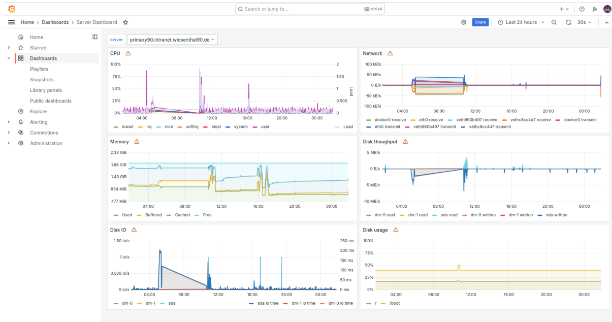
Fig. 15.2: Server dashboard
