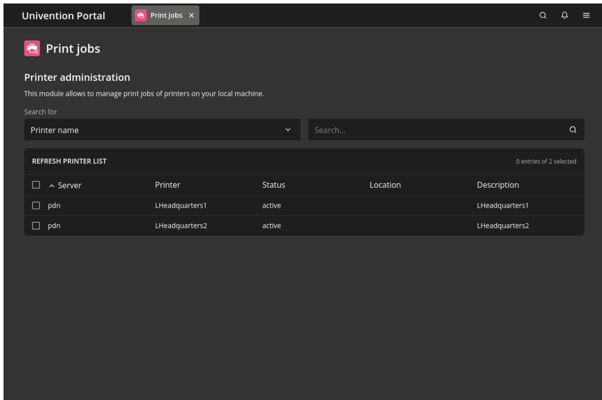
Fig. 13.2: Printer administration
