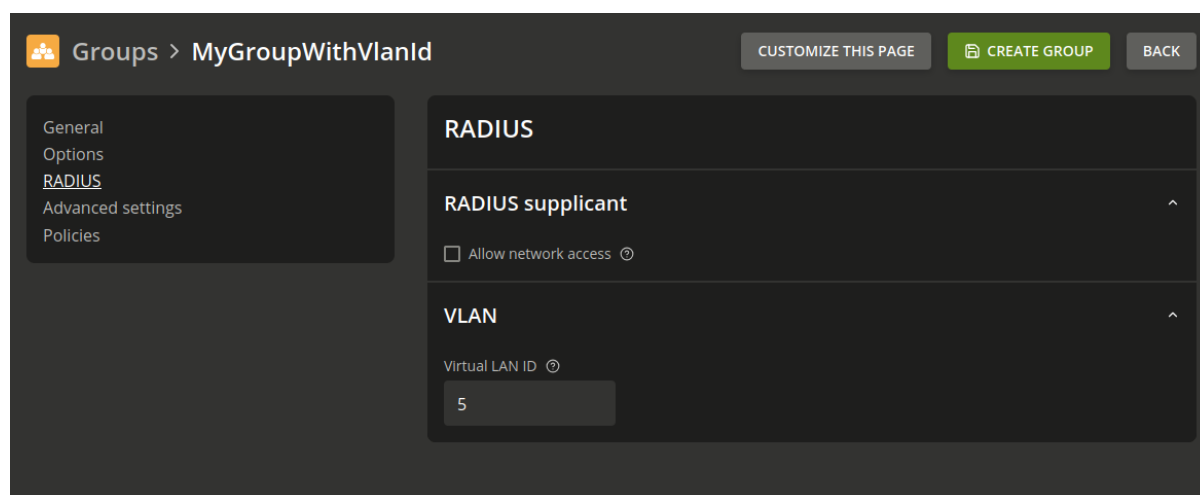
Fig. 11.8: Assigning VLAN ID to a user group
